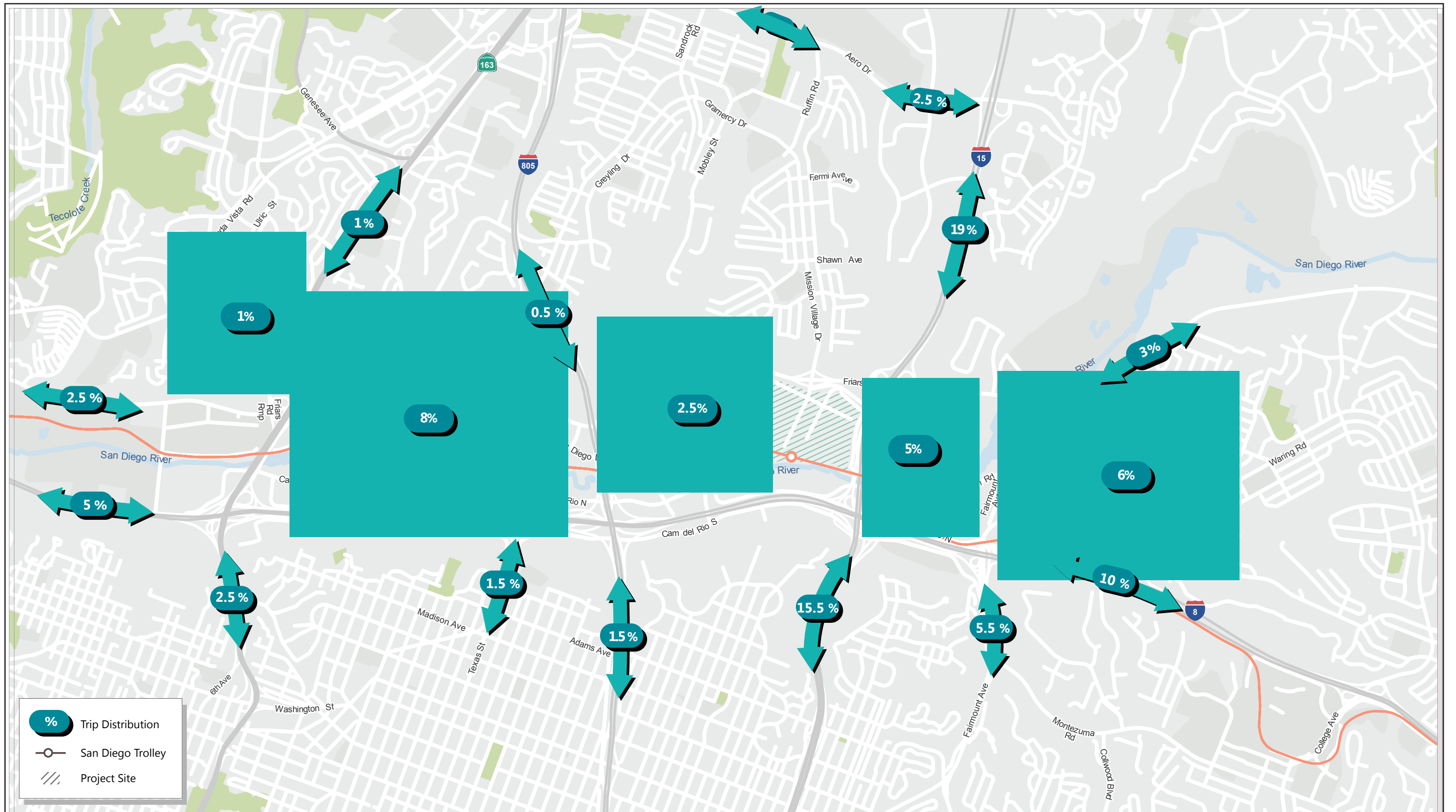
Figure 4.15-6 Trip Distribution
